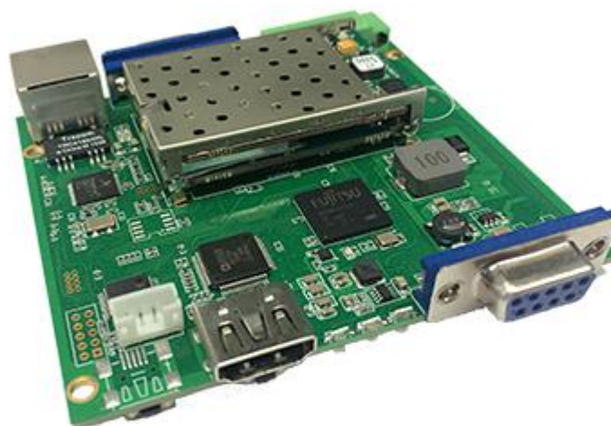
Low Delay Network High Definition Video Codec Board 9.5x9x1.5cm,85g
