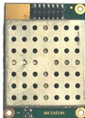
SDR400M 65x36x13mm,25g
