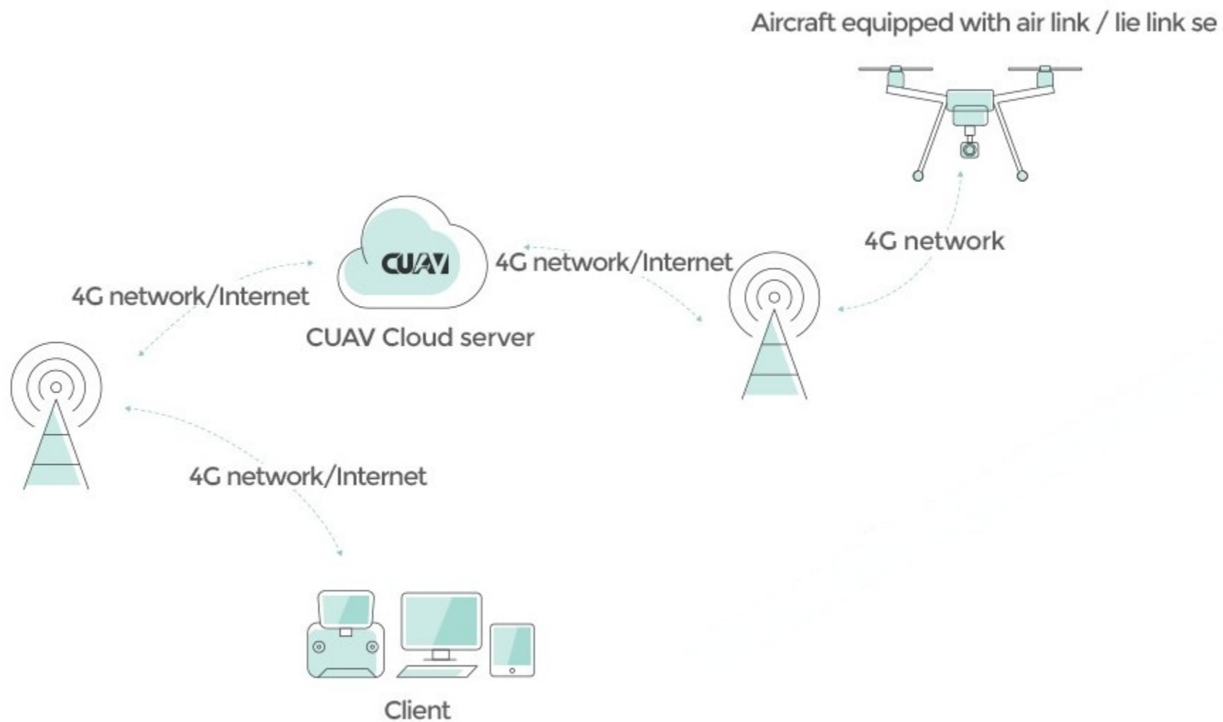
Working principle diagram of LTE Link series products
