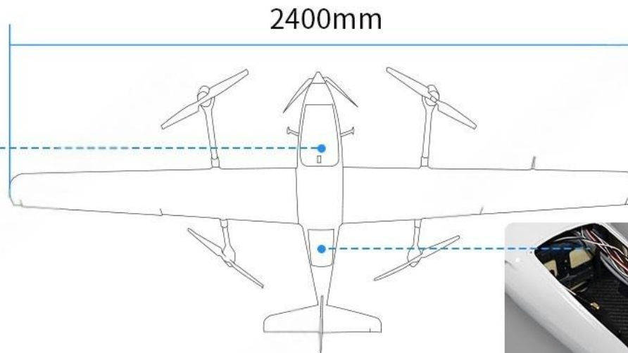
Battery compartment: 20 \times 9 \times 6\text{cm}
